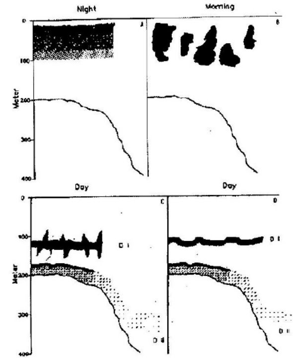
Figure 2 Typical echo sounder of mesopelagic fish in the Gulf of Oman A: night; B: morning; D and D: day time
